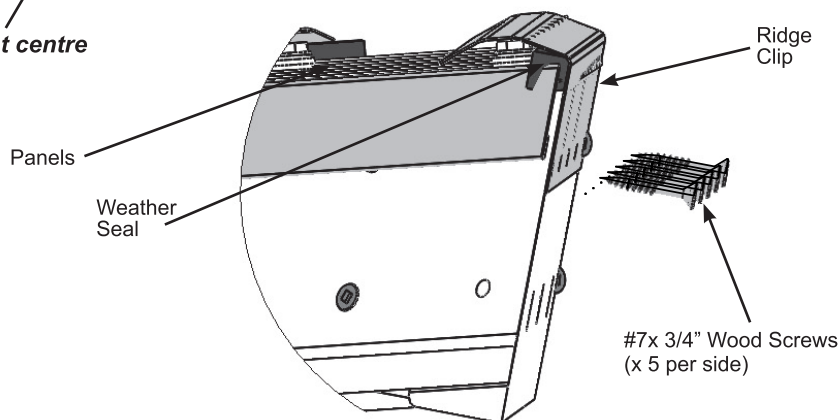
Fig. 10.4 Side View
